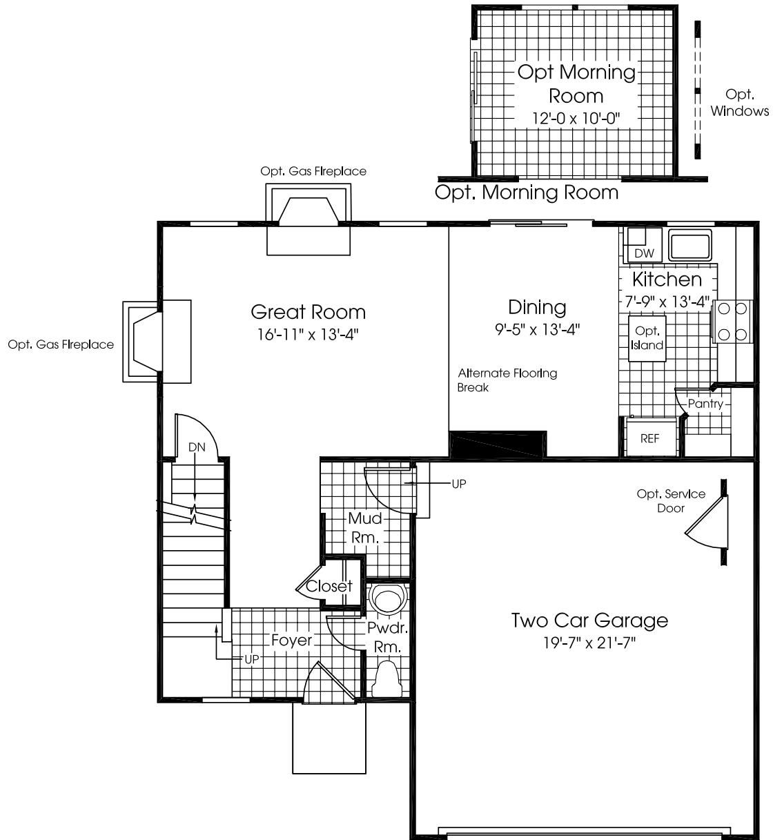
MAIN LEVEL ELEVATION C
